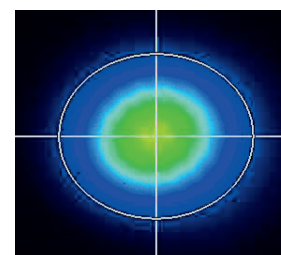
Typical beam intensity profile (20 cm from laser output) of MPL1310-DP series lasers
